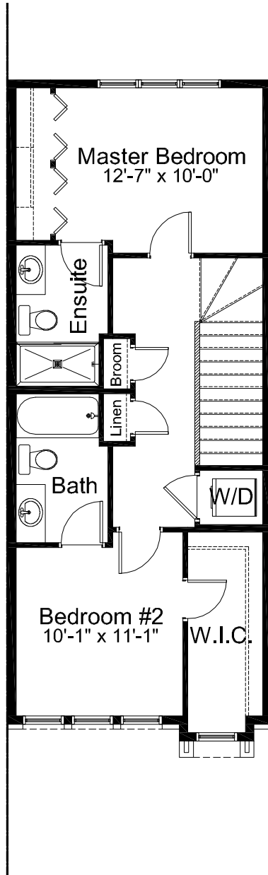
UPPER FLOOR - BASE PLAN 629 SQ FT
