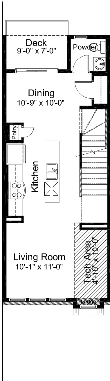
MAIN FLOOR - BASE PLAN 577 SQ FT
