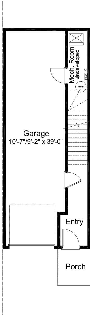
LOWER FLOOR - BASE PLAN
