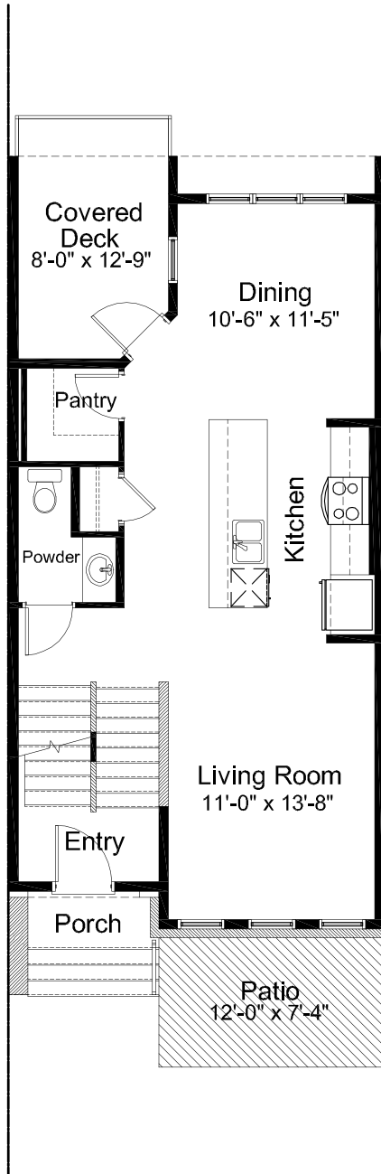
MAIN FLOOR - BASE PLAN 690 SQ FT
