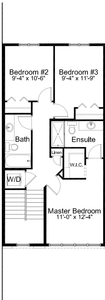
UPPER FLOOR - BASE PLAN 777 SQ FT
