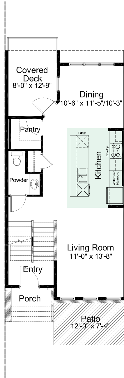
MAIN FLOOR - GOURMET KITCHEN OPTION 690 SQ FT WALL OVEN/MICROWAVE HOOD FAN COOKTOP BAR FRIDGE
