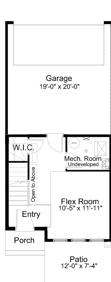
LOWER FLOOR - BASE PLAN 267 SQ. FT. PATIO: 88 SQ.FT.
