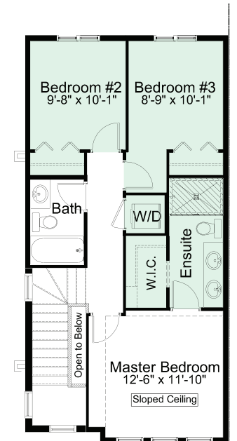
UPPER FLOOR 3 BEDROOM OPTION 705 SQ. FT.
