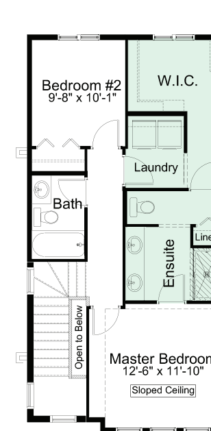
UPPER FLOOR 2 BEDROOM OPTION W/ WALKTHROUGH LAUNDRY 705 SQ. FT.
