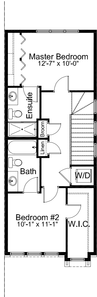
UPPER FLOOR - BASE PLAN
