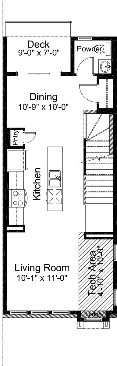
MAIN FLOOR - BASE PLAN
